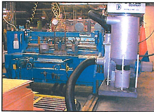
Cyclone dust collector mounted on press, provides low maintenance, high flow, clean dust containment
