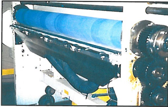
Sheet Cleaner is located after the infeed rollers, before first print station, to clean the printed side of sheet
